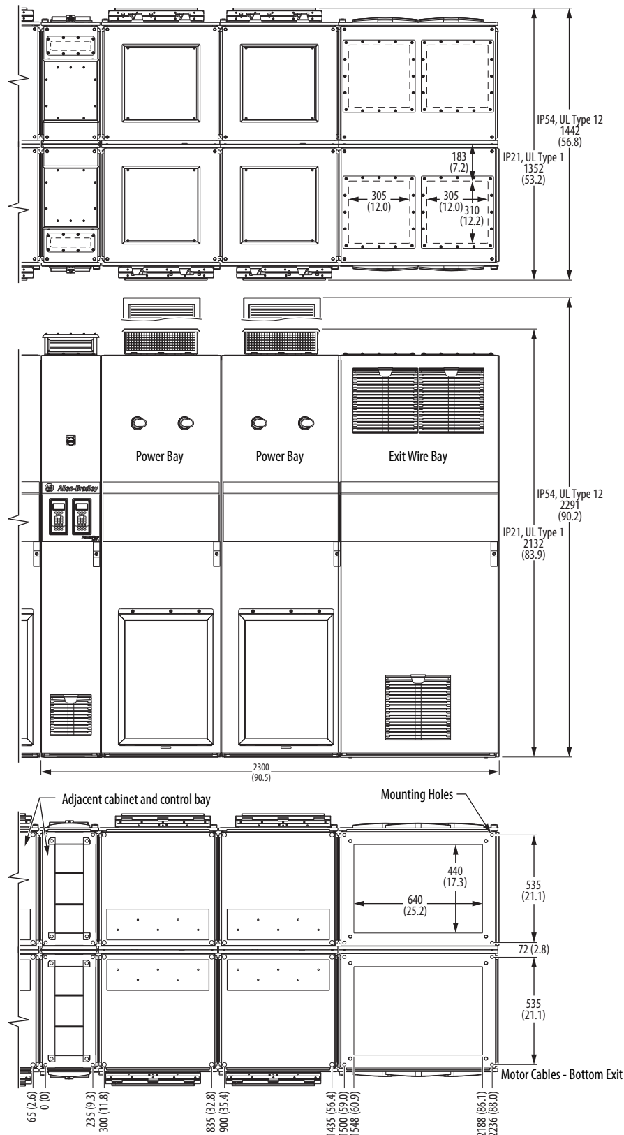
Frame 14 Common Bus Inverters Top, Front, and Bottom Views - Dimensions are mm (in.)
