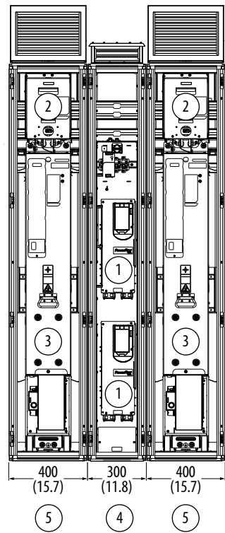
Two Frame 8 Common Bus Inverters with Common Control Bay
