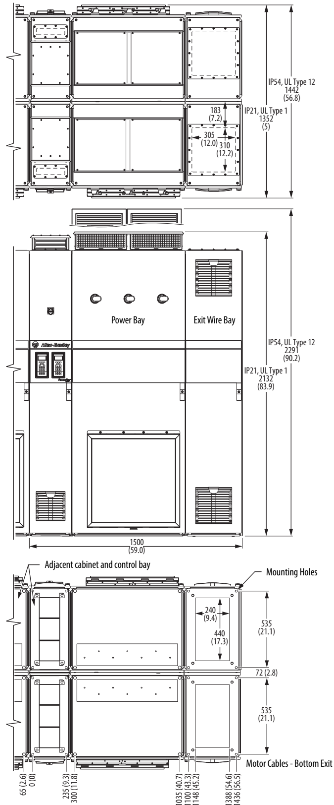
Frame 13 Common Bus Inverters Top, Front, and Bottom Views - Dimensions are mm (in.)
