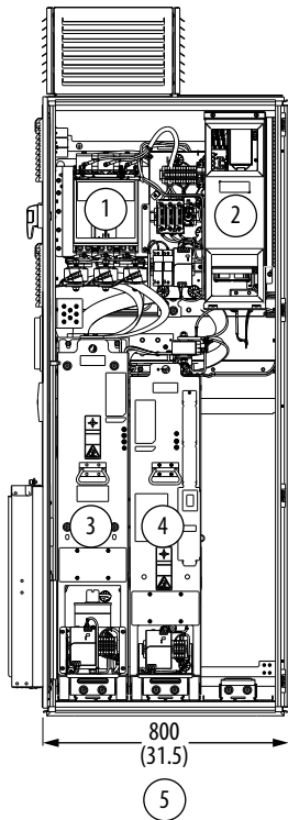
All cabinet enclosures are 600 mm (23.6 in.) deep. Frame 7 IP54, UL Type 12 Enclosure Shown.
