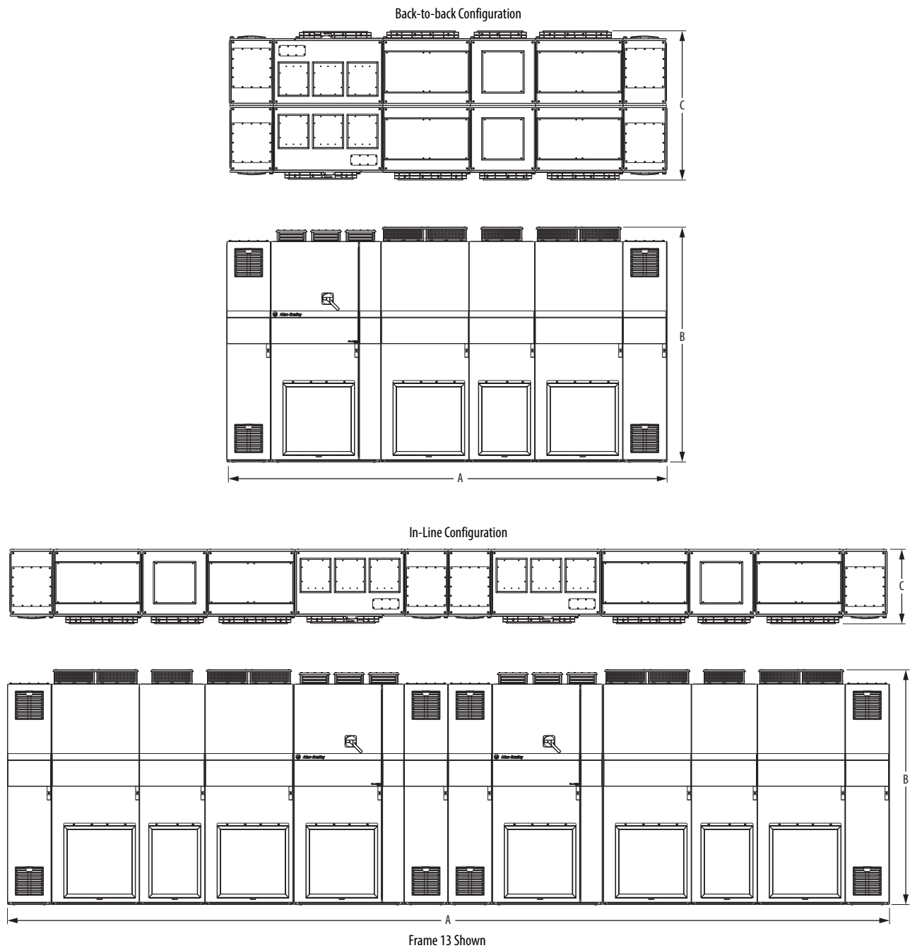
Frame 13...15 Drives Top and Front Views - Dimensions are mm (in.)
