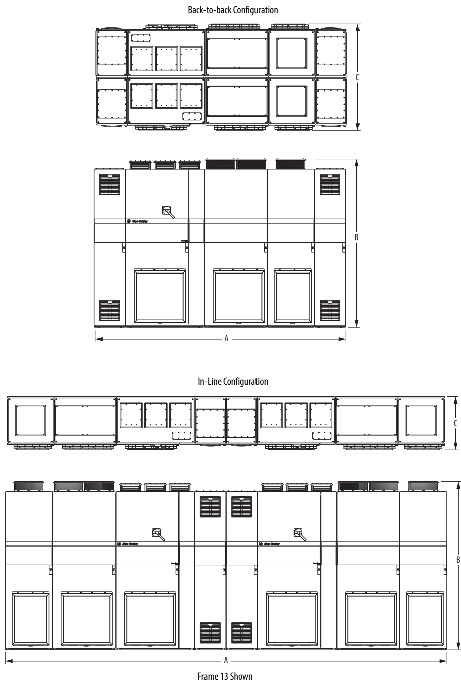
Frame 13...15 Bus Supplies Top and Front Views - Dimensions are mm (in.)
