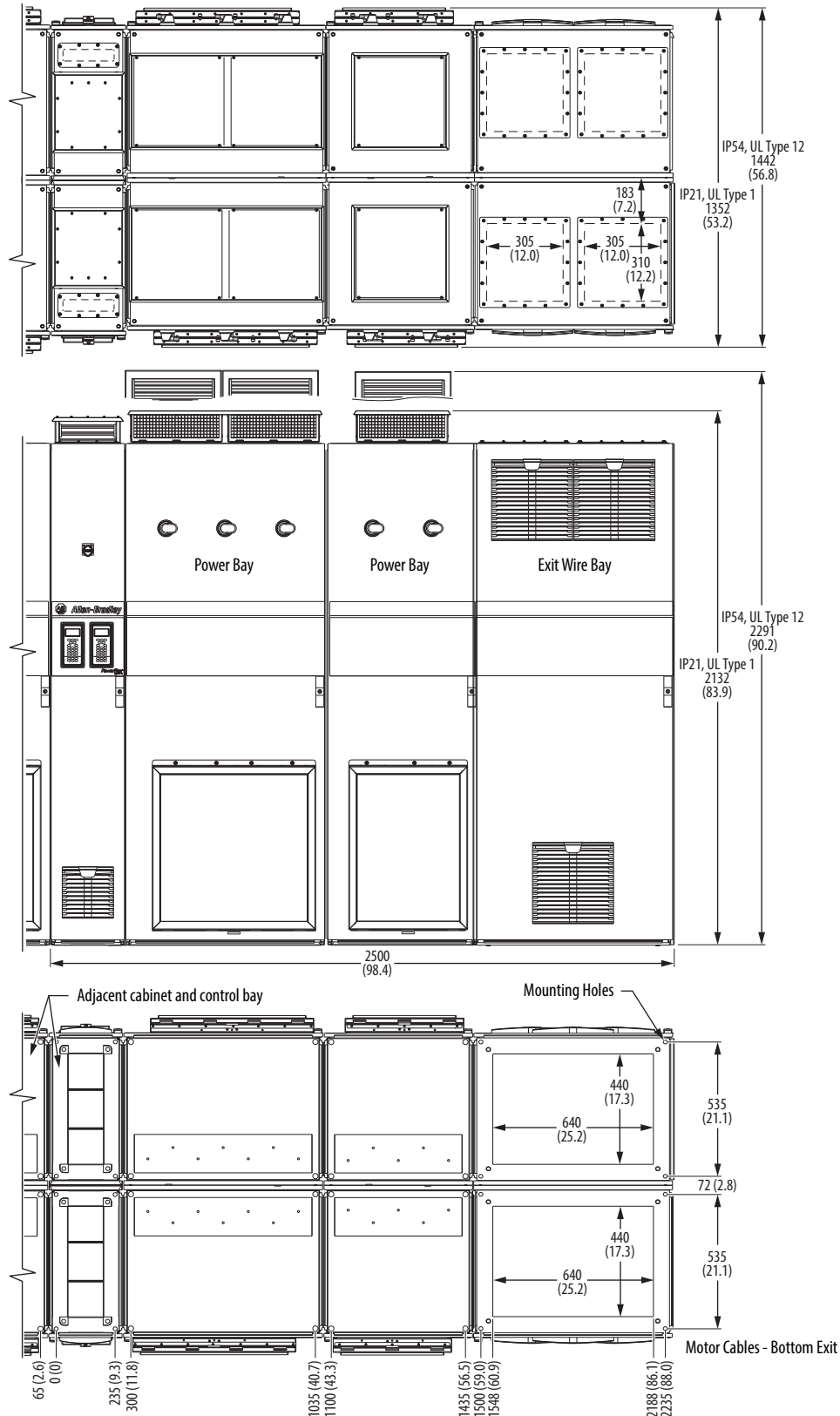
Frame 15 Common Bus Inverters Top, Front, and Bottom Views - Dimensions are mm (in.)
