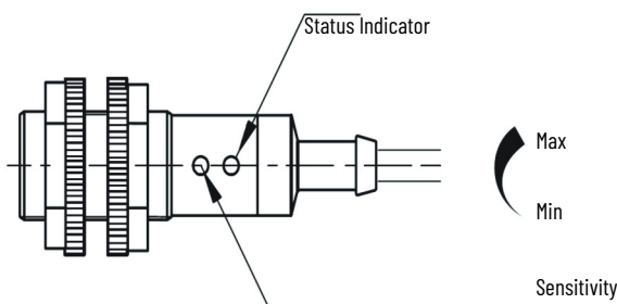
Figure 2 - M30 Housing
