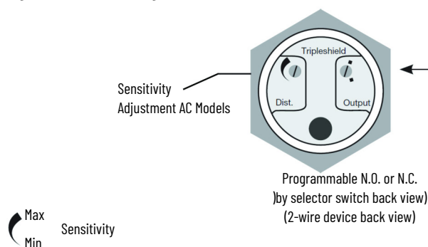
Figure 2 - M30 Housing
