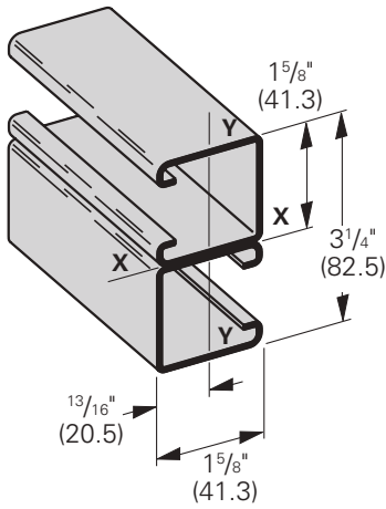
B24C Wt. 2.80 Lbs./Ft. (4.16 kg/m)
