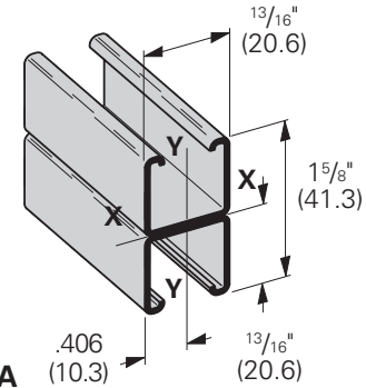
B62A Wt. .84 Lbs./Ft. (1.25 kg/m)
