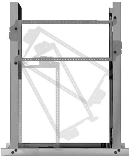
Telescoping bracket
