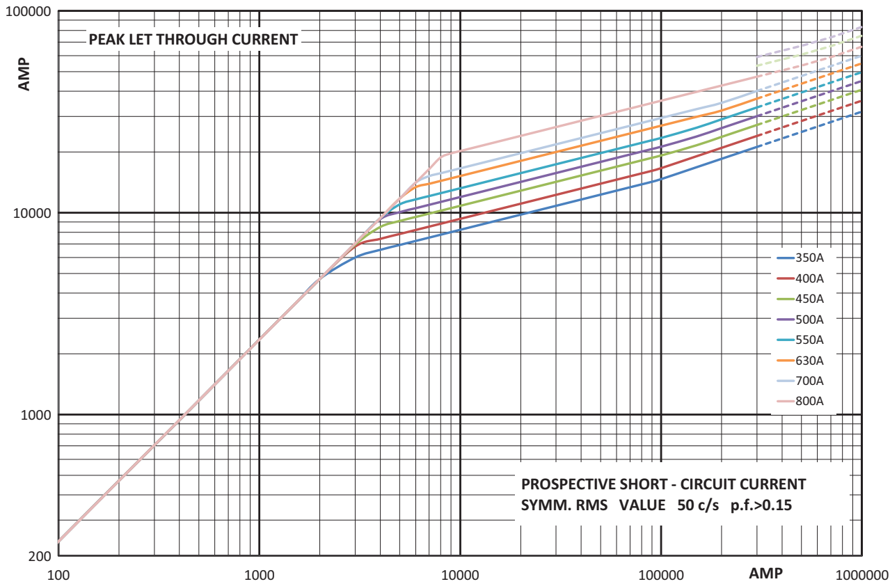
Cut-off curve - Size 3, 350 A to 1000 A
