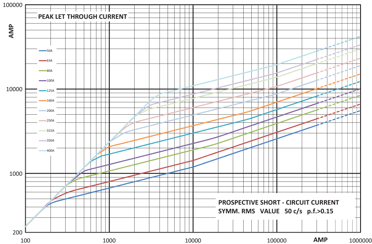
Cut-off curve - Size 1*, 50 A to 400 A
