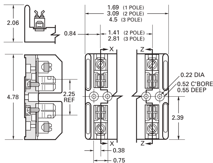
Figure 2. 61 to 100 A
