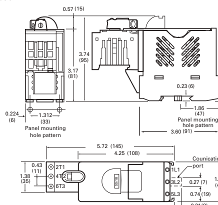
OPM-1038SW
