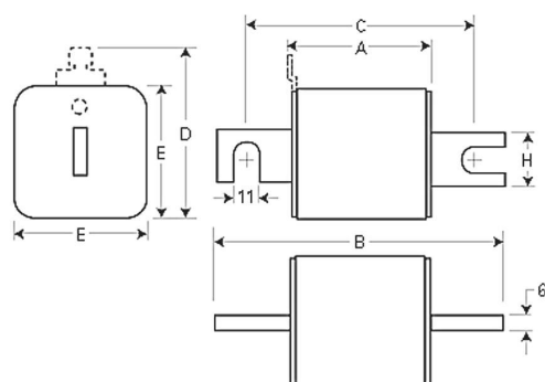
Type -110-TN/110
