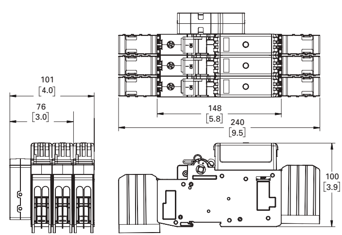
100 amp switches
