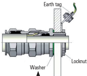
WITH WASHER: IP66 / IP68
