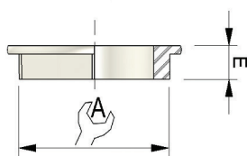
Ordering codes - Locknut
