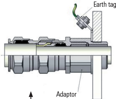
CABLE GLAND WITH ACCESSORIES
