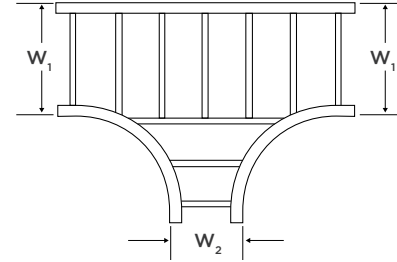
HORIZONTAL EXPANDING TEE W 1 > W 2
