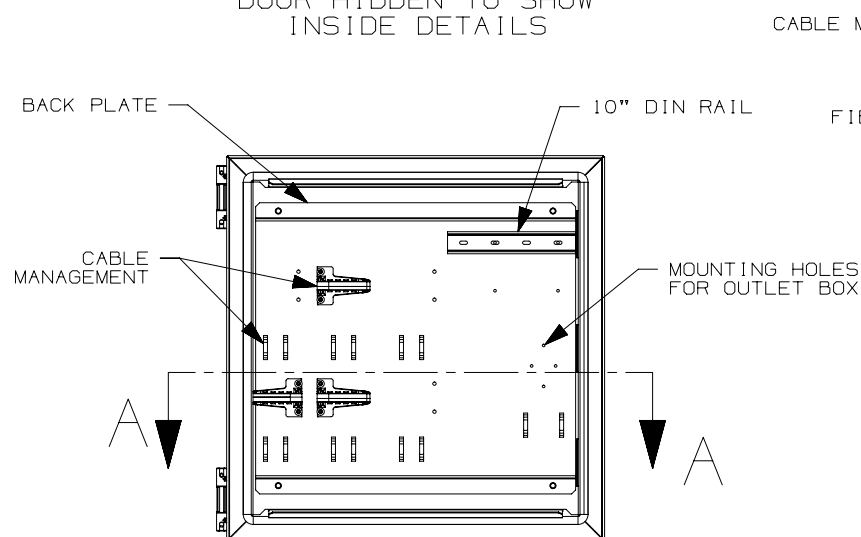
FRONT VIEW SHOWING BACK PANEL
