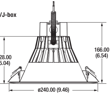
3000lm w/J-box
