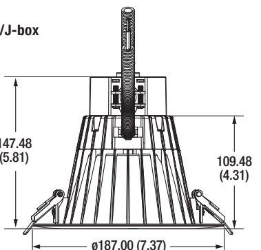
2000lm w/J-box
