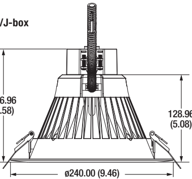
5000lm w/J-box
