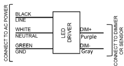
Wiring Diagram 2
