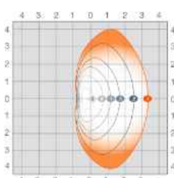
AREAFLD2A-240W-T5 at 45° tilt
