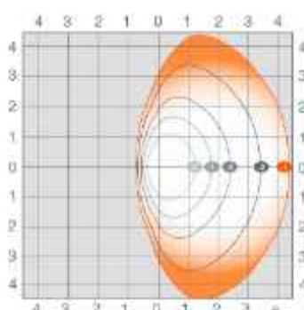
AREAFLD2A-240W-T3 at 45° tilt
