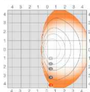
AREAFLD2A-150W-T4 at 45° tilt
