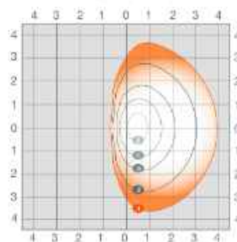
AREAFLD2A-80W-T4 at 45° tilt
