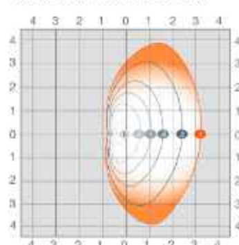
AREAFLD2A-100W-T5 at 45° tilt
