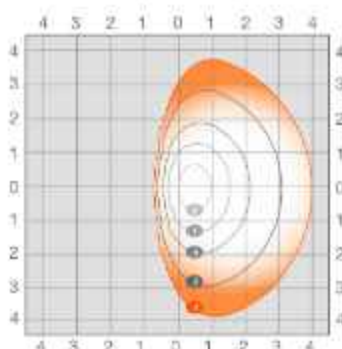
AREAFLD2A-200W-T4 at 45° tilt
