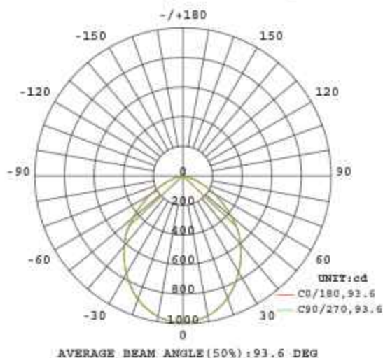
Zonal Lumen Distribution
