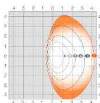
AREAFLD2A-100W-T3 at 45° tilt
