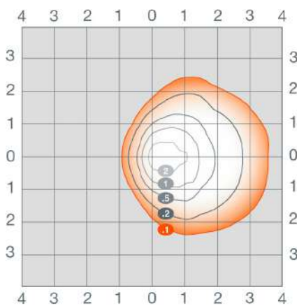
WALPAK4A 120W
