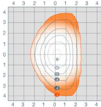
AREAFLD2A-200W-T3
