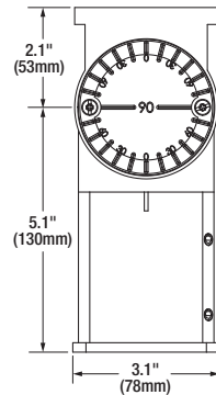
Round Pole Adapter (60128)
