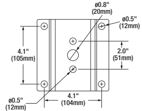
Wall Mount (60129 or 60652)
