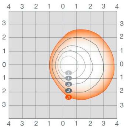
WALPAK4A 80W
