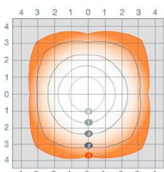
AREAFLD2A-240W-T5
