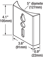
Wall Mount (60129 or 60652)
