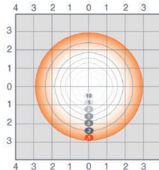
45W CANOPY2A45UNVD840 Isofootcandle Lines at 10' Mounting Height
