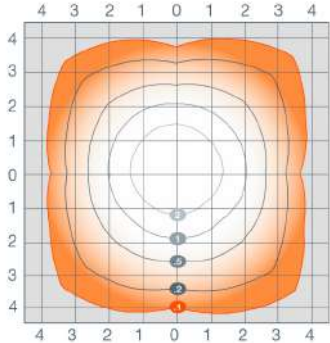
AREAFLD2A-150W-T5
