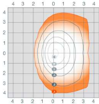
AREAFLD2A-200W-T4
