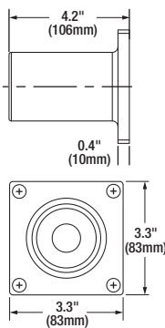
Round Pole Adapter (60128)
