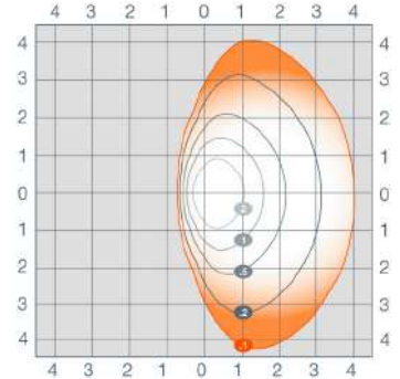
AREAFLD2A-200W-T3 at 45° tilt
