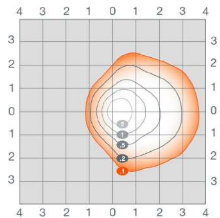
WALPAK4A 60W
