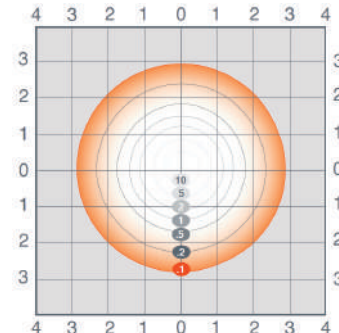
65W CANOPY2A65UNVD840 Isofootcandle Lines at 10' Mounting Height
