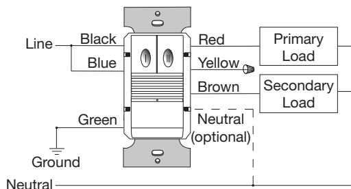
PW-302 and PW-302-347 Bi-Level Wiring
