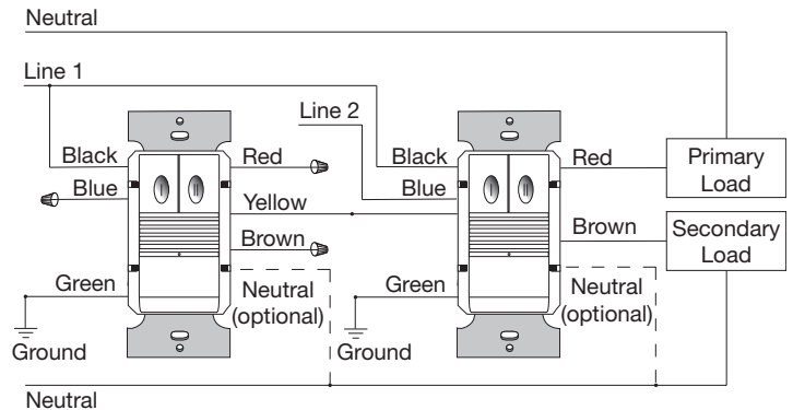
Two-phase Wiring
