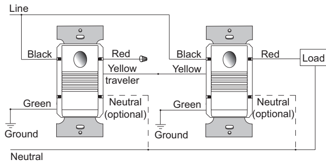
Typical Wiring (PW-301 or PW-301-347 up to 4 sensors)
