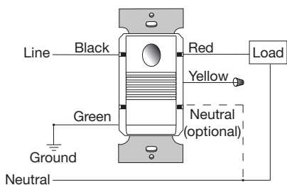
PW-301 and PW-301-347 Wiring
