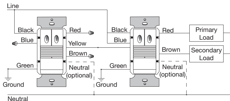
Bi-level Wiring (PW-302 or PW-302-347 up to 4 sensors)
