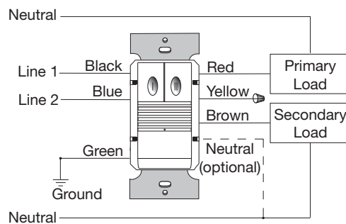
PW-302 and PW-302-347 Dual Circuit Wiring
