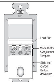
Fig. 5: Sensor Adjustment Controls
