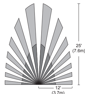
Fig. 1: Sensor Coverage Area
